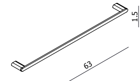
LOFT Towel Rail AR33001
