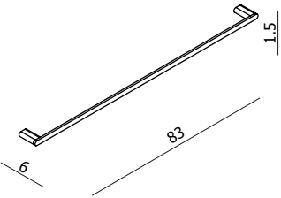
LOFT Towel Rail AR33014
